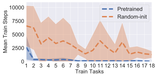
(a) With feedback from evaluating the compositional policies in the environment, compares the effect of pretraining on the number of training steps needed to learn each translation from each mission to each Boolean expression
