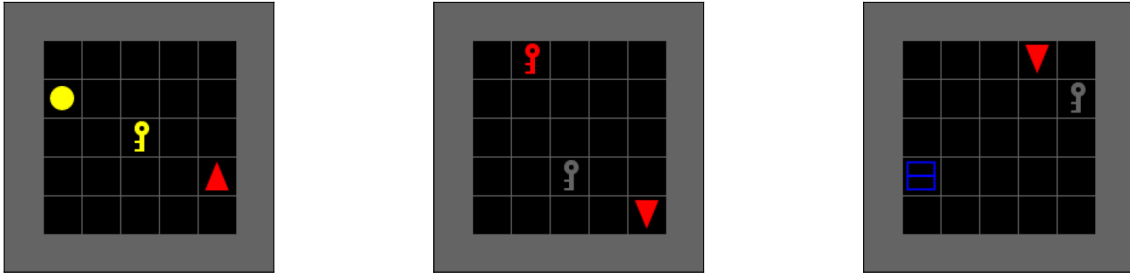
(a) Language command “pick up the yellow ball” with corresponding logical expression \text{pickup\_yellow} \wedge \text{pickup\_ball} . (b) Language command “pick up the red key” with corresponding logical expression \text{pickup\_red} \wedge \text{pickup\_key} . (c) Language command “pick up the blue box” with corresponding logical expression \text{pickup\_blue} \wedge \text{pickup\_box} .
