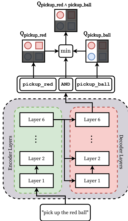
Figure 2: The T5-small model first translates the input mission command “pick up the red ball” into a Boolean expression, with variables representing the vocabulary of possible compositional value functions. Then the intersection of the value functions is computed, resulting in a value function for picking up a red ball in the environment.
