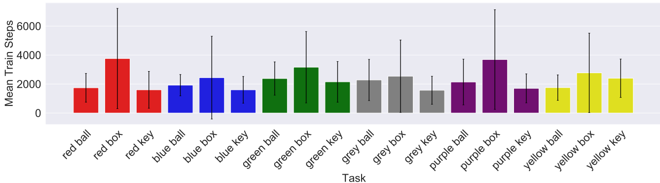
Figure 4: The mean training steps needed to learn the translation from each mission to each Boolean expression for each of the 18 potential tasks, when the translation model has perfect feedback from the environment. Rewards are +1.0 for equivalent output Boolean expressions and -1.0 for incorrect expressions. Means and Standard Deviations computed over 10 trials.
