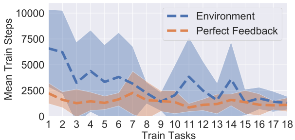
(c) With a randomly-initialized T5 model, compares the learning of the agent from policies evaluated in the environment to “perfect” feedback based only on the output Boolean expression.
