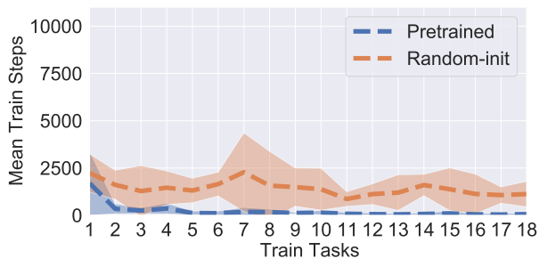
(b) With “perfect” feedback based only on the output Boolean expression, compares the effect of pretraining on the number of training steps needed to learn each translation from each mission to each Boolean expression.
