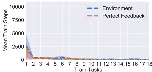
(d) With a pretrained T5 model, compares the learning of the agent from policies evaluated in the environment to “perfect” feedback based only on the output Boolean expression.
